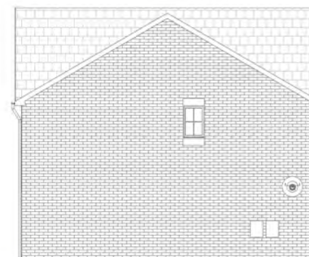
PLOT 48 SIDE ELEVATION
