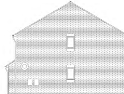
PLOT 53 SIDE ELEVATION
